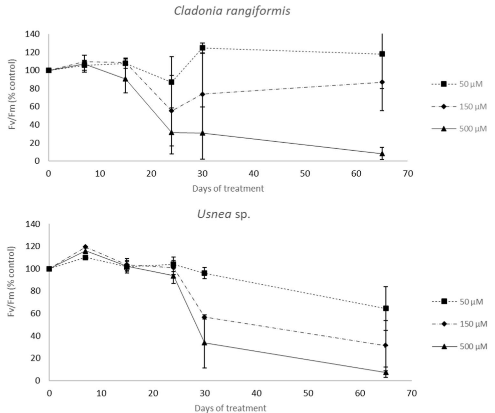
Fig. 2 Fv/Fm values (% of the control, mean value, n=5) in Cladonia rangiformis and Usnea sp. Squares = 50 \mu\text{M} \text{NH}_4\text{Cl} ; diamonds = 150 \mu\text{M} \text{NH}_4\text{Cl} ; triangles = 500 \mu\text{M} \text{NH}_4\text{Cl} . Vertical bars represent standard deviation
