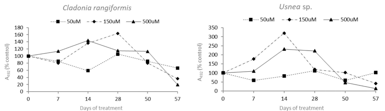
Fig. 3 Viability of the mycobiont as indicated by TTC reduction: Values of absorbance at 492 nm (% of the control) in Cladonia rangiformis and Usnea sp. Squares = 50 \mu\text{M} \text{NH}_4\text{Cl} ; diamonds = 150 \mu\text{M} \text{NH}_4\text{Cl} ; triangles = 500 \mu\text{M} \text{NH}_4\text{Cl}
